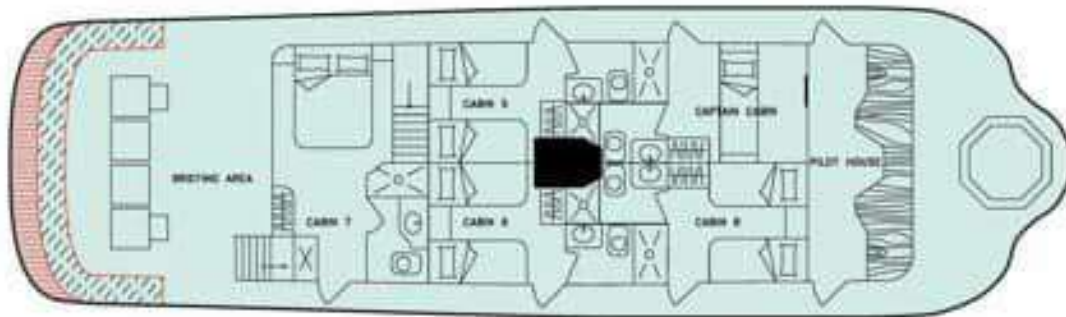
LEVEL THREE
