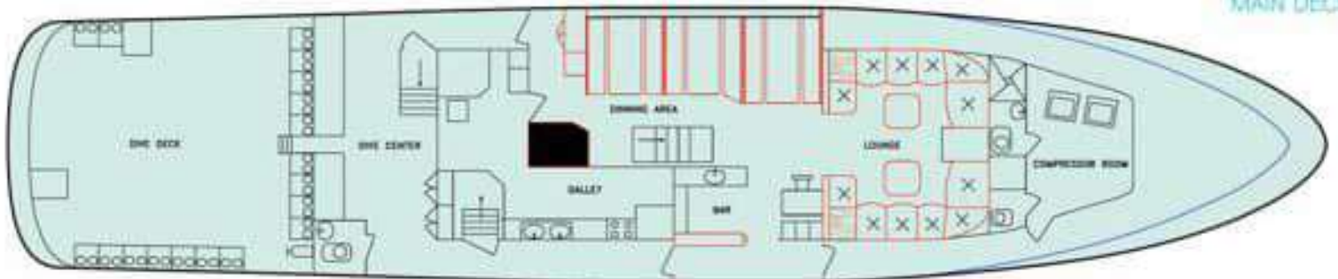
MAIN DECK
